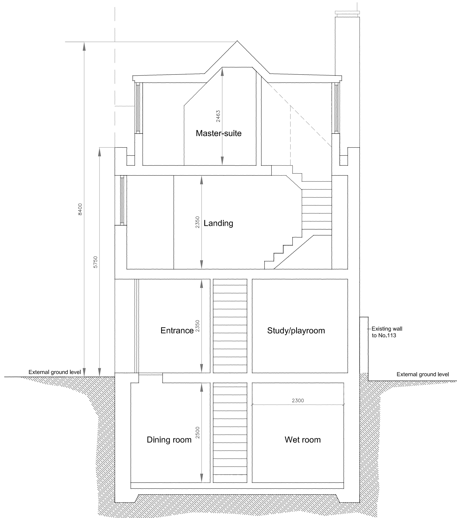
Section B SCALE 1-50@A3
